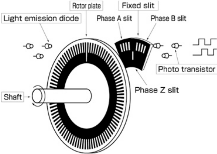
Incremental Encoder Simplified Structure
